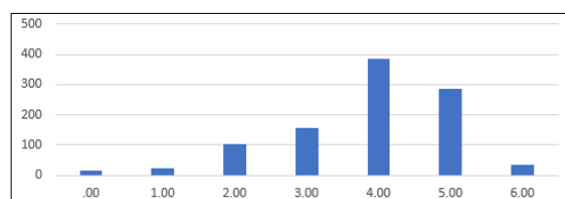
Figure 4. HHS distribution.
