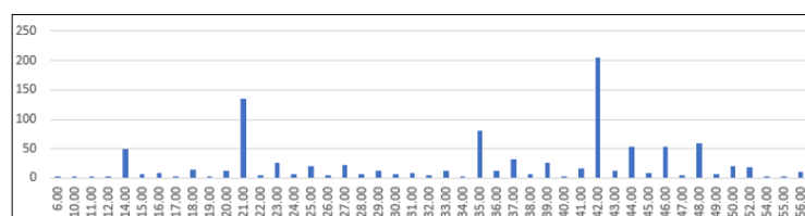
Figure 3. rCSI distribution.
